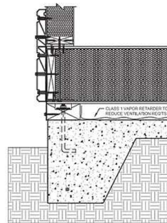
CONCRETE SLAB
