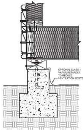
CONCRETE STRIP FOOTING
