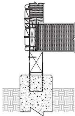
WOOD BEAM ON CONC. PIERS
