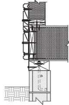
CMU WALL
